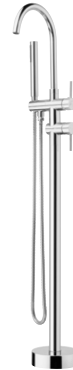
Floor Mounted Minimal Bath Mixer with Handshower (MP) (10) Min. Pressure 150kPa WELS: Mains 3 Star; 8L/min Spout Height: 1080mm Spout Reach: 200mm Product code: BF95CH
